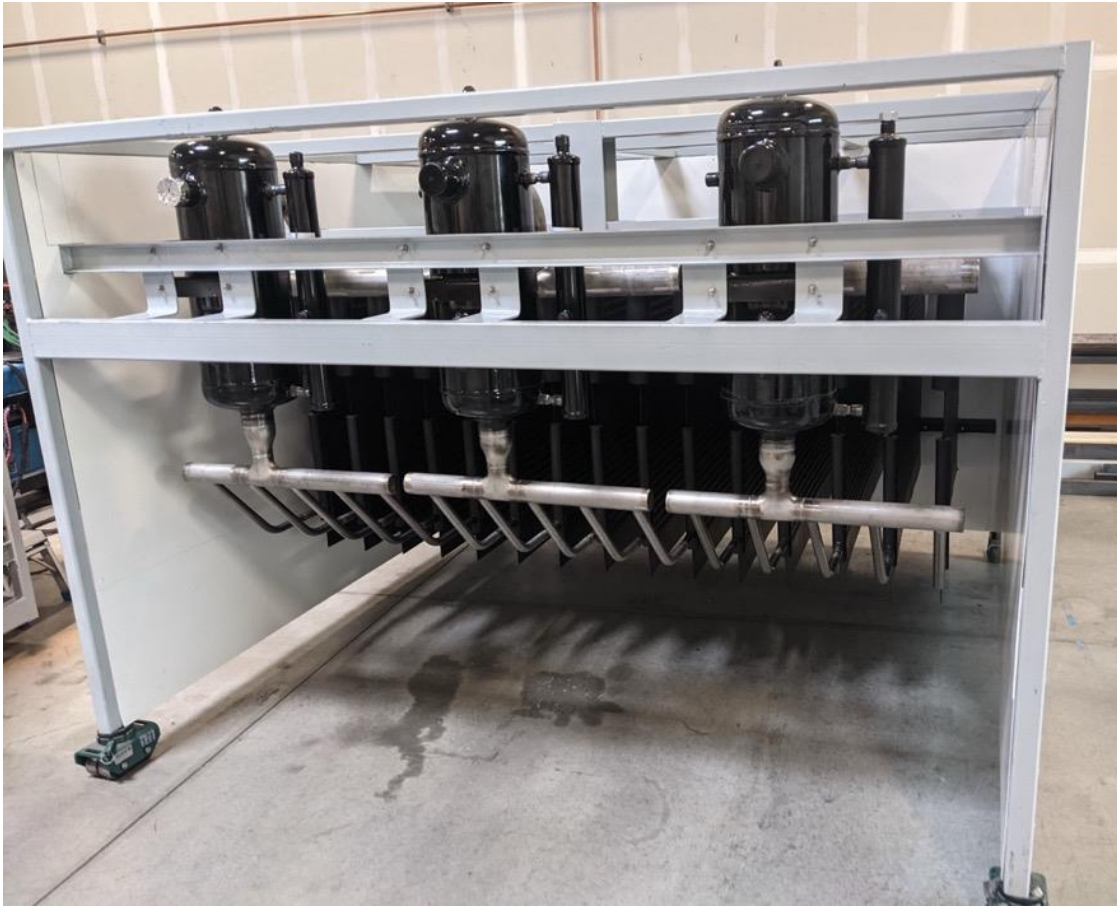
Figure 6: A 60,000lb/day ice making module ready for hookup to refrigerant feed.
